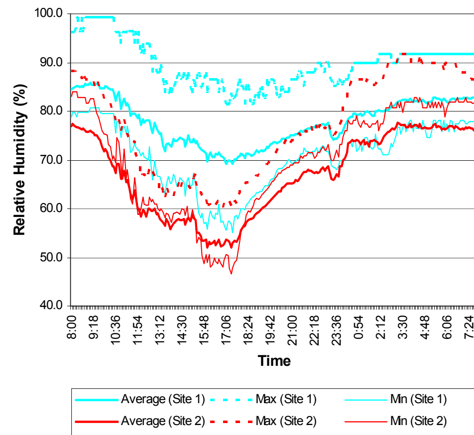
Fig. 4: Comparison of the relative humidity between the two sites
