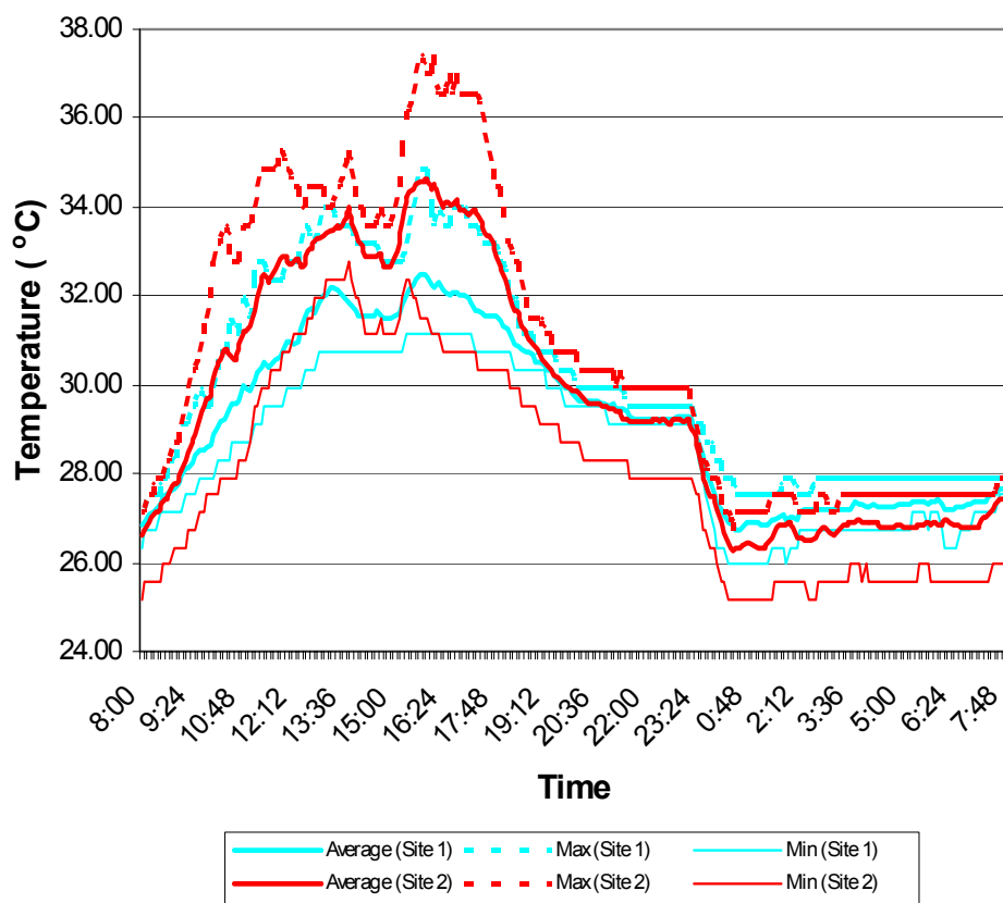
Fig. 3: Comparison of the ambient air temperature between the two sites
